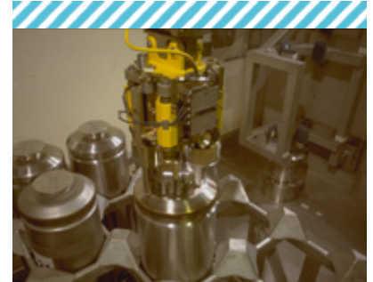
Example of packages of compacted ILW-LL (intermediate level, long-lived): technological waste, hulls and end-pieces
